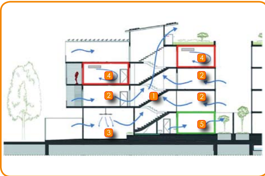
Natural ventilation of the town house (Source: Schwede, Hesse 2010)
