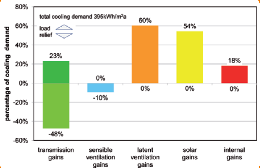
Cooling demand of a typical town house, when mechanically conditioned (simulation result; Source: Schwede 2009)
