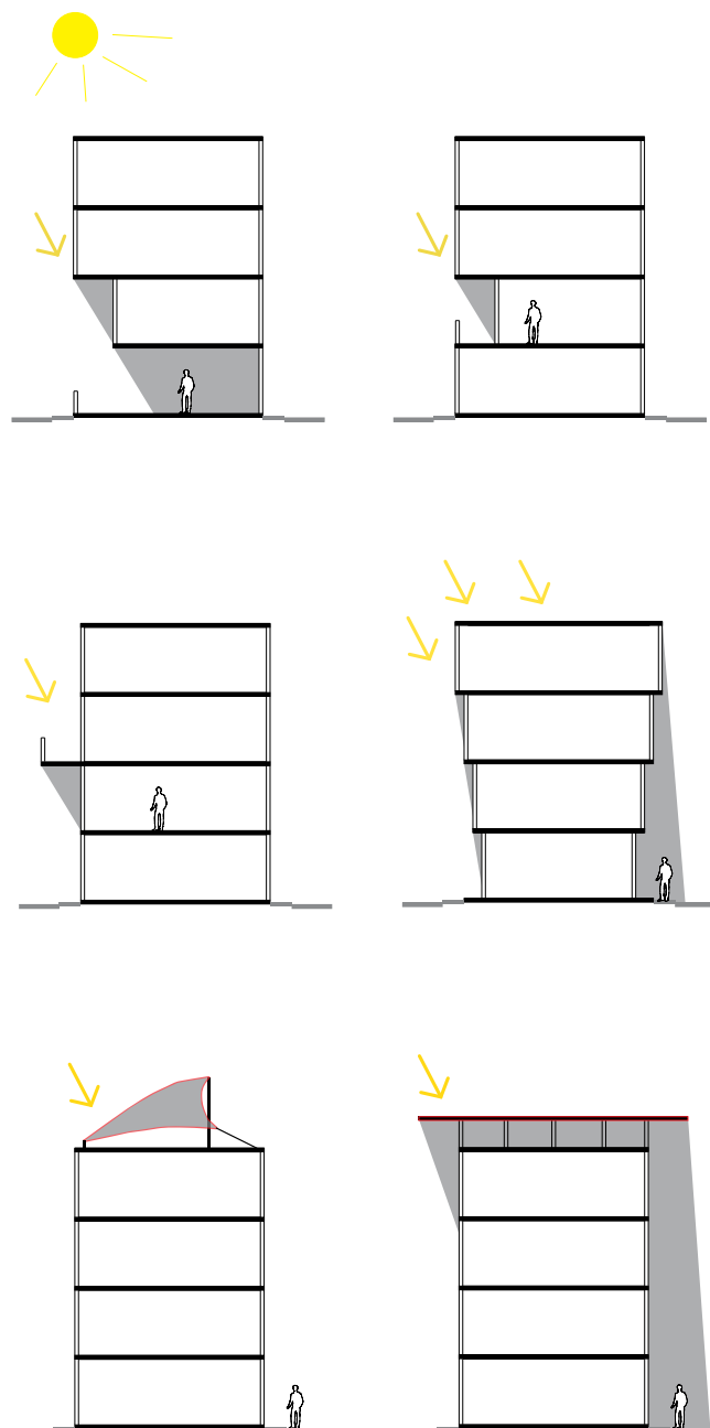
Constructive sun protection methods (Source: Hesse 2009)
