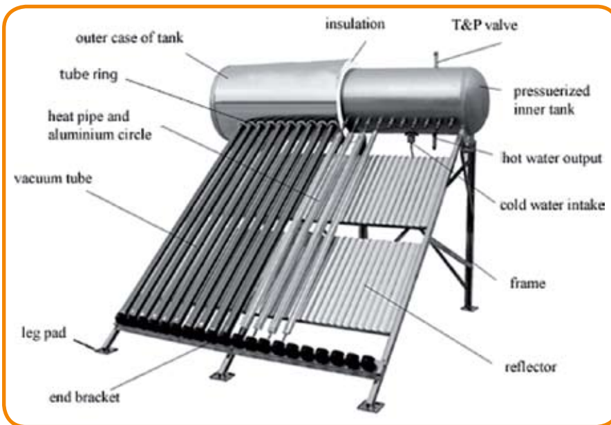
Components of a solar water heating device (Source: Nhien 2010)
