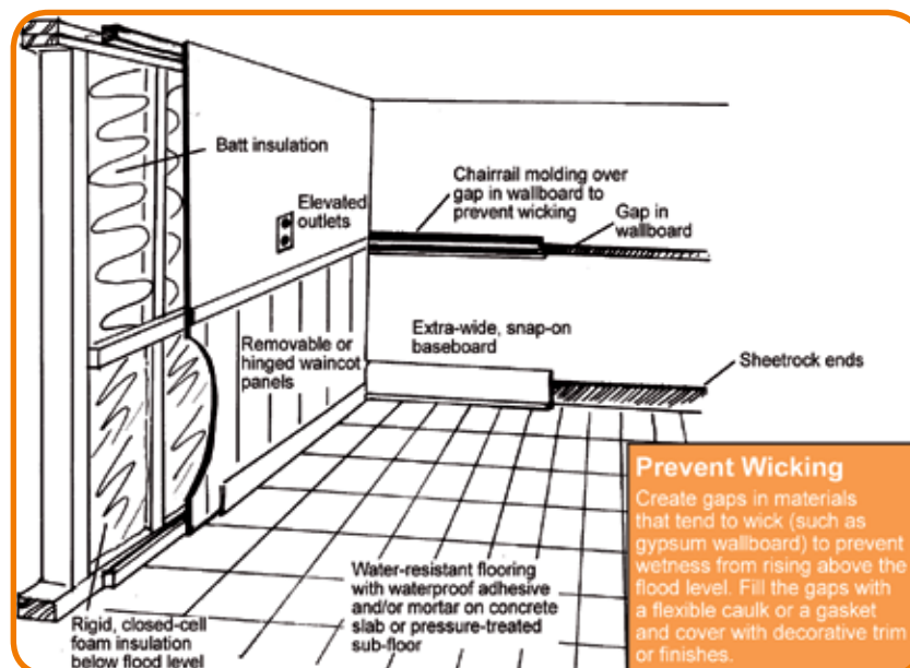
Wet flood-proofed walls and floors (Source: www.lsuagcenter.com )
